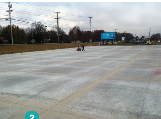
Sawing control joints
